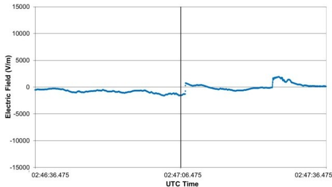
Figure 17. 10/10/2011 02:47:06.475 UTC -1525 V/m E-field measured 1.199 km from Stroke
