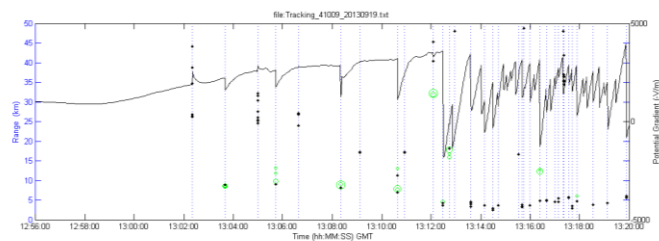
Figure 12b. 9/18/13 storm passage where the corona effect was noted between 1300 and 1400 GMT.
