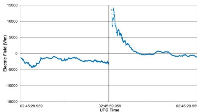
Figure 15. 10/10/2011 02:45:59.959 UTC -3376 V/m E-field measured 4.104 km from Stroke
